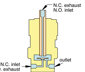
3-Way N.C. Manifold Mount
