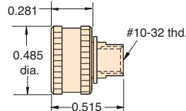
Part No. MIQC-CFT Description #10-32
