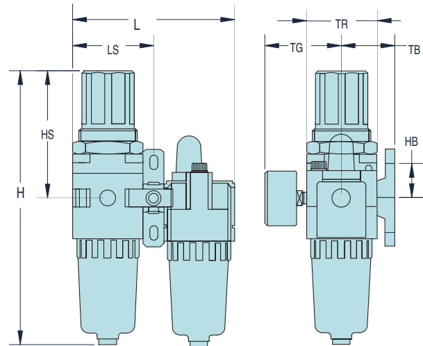
MMFRS-3Q-D Stacking FRL with Bowl Shields and Automatic Drain
