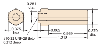
11675-12 3/8" O.D. Tube
