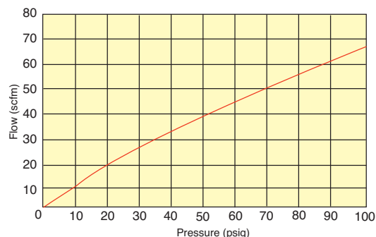
Pressure vs. Flow
