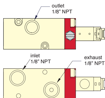
Mounting Interface
