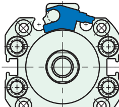
1 1/16" Bore
