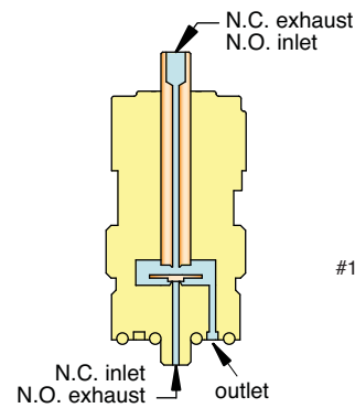
3-Way Fully-Ported Manifold Mount
