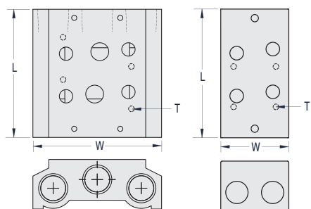
4-Way Manifold
